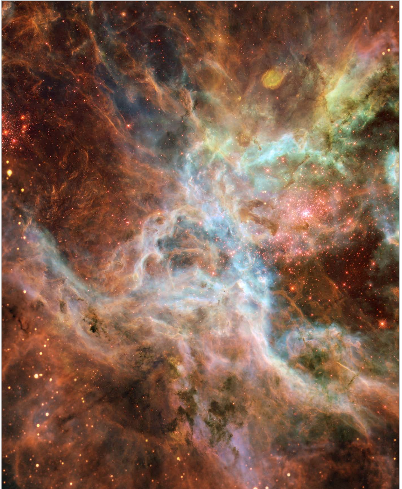
The Tarantula Nebula, also known as 30 Doradus, is a hotbed of star-formation situated 170,000 light-years away in the Large Magellanic Cloud (LMC) in the Southern sky. Just to the right of centre of the image there is a huge cluster of very hot young stars called R136.
