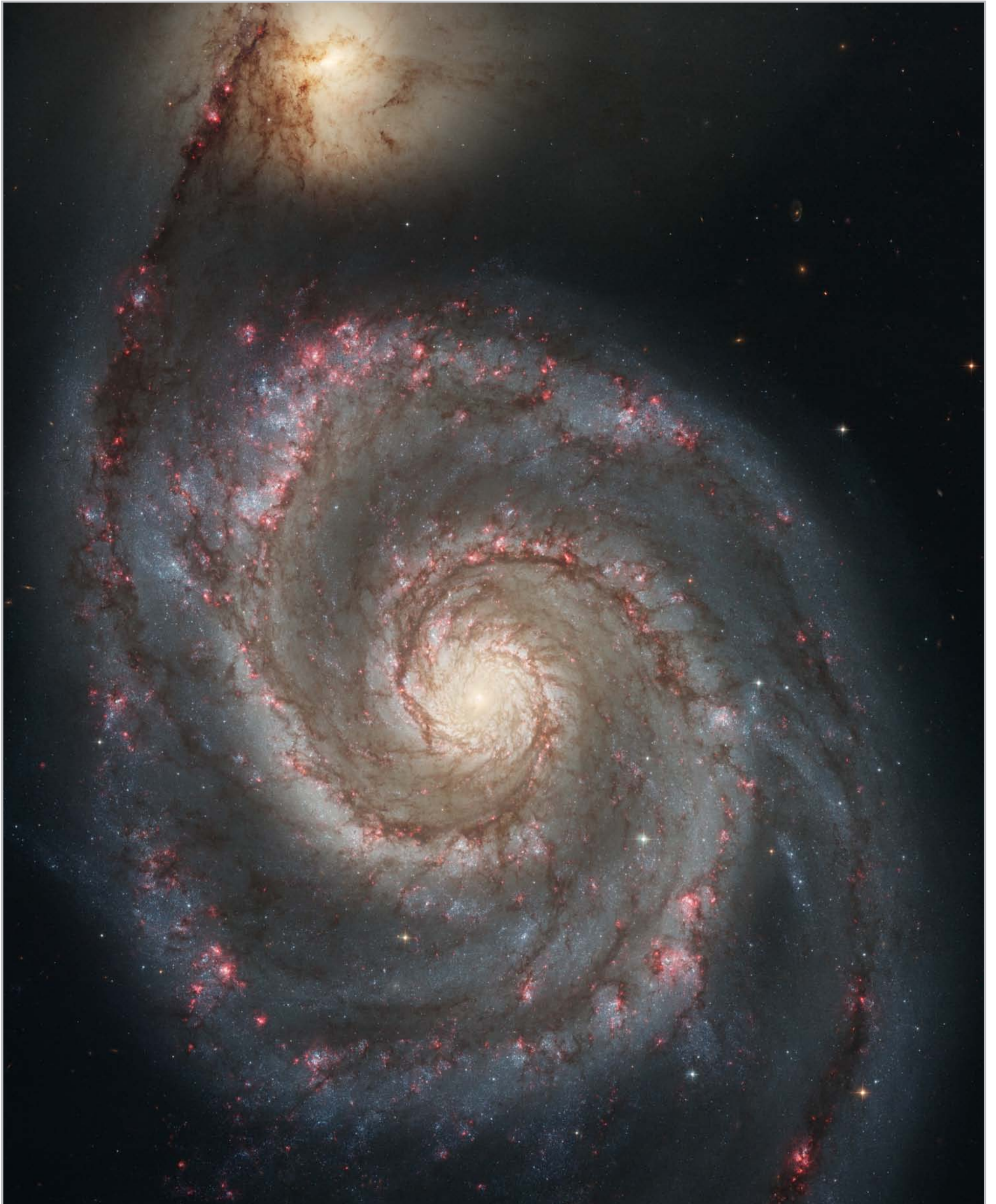
The graceful, winding arms of the majestic spiral galaxy M51 (NGC 5194) appear like a grand spiral staircase sweeping through space. They are actually long lanes of stars and gas laced with dust.
